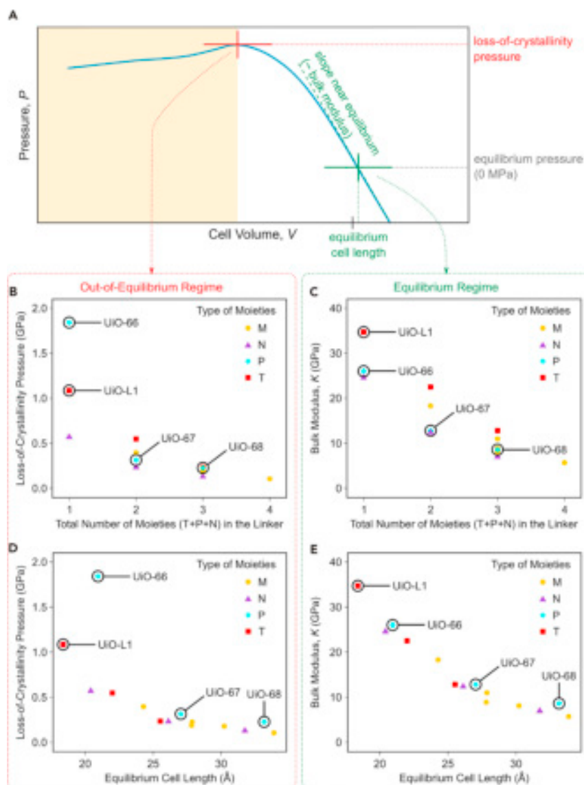
Figure 5. Probing MOF Stability Using In Operando Molecular Dynamics
