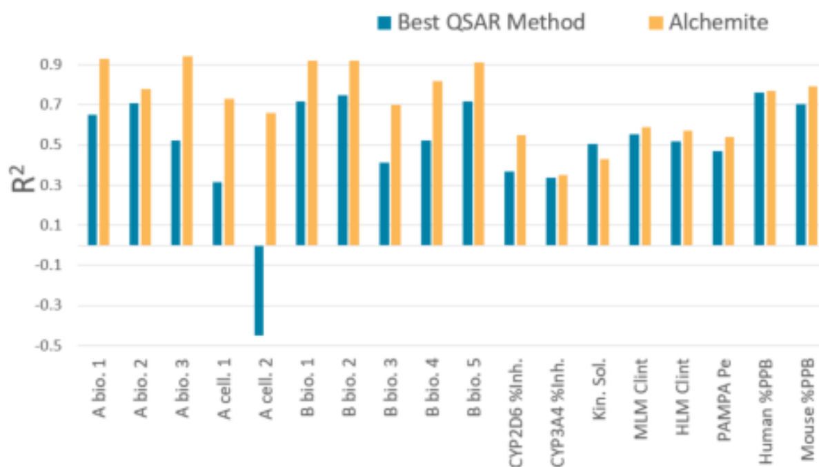
Figure 9. Comparison of the results on the independent test set for best of four QSAR methods (blue) with an Alchemite model (orange) built with all of the training data using an 80:20 stratified random split on the final data set. This plot can be compared to Figure 2 to inspect the improvement in models with more data.
