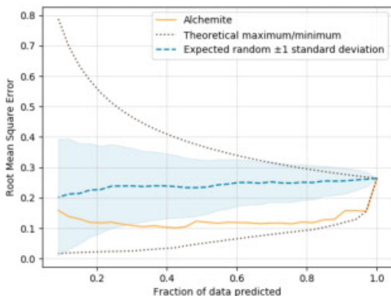
Figure 5. Plot of RMSE of predicted test results when predictions with lowest confidence are removed. The orange line shows the performance of the Alchemite model. For comparison, the black dotted lines show the minimum and maximum RMSE achievable as the least- and most-accurate results are removed, i.e. the order which minimizes or maximizes the RMSE (N.B. in practice this order is not known without measuring against the test set). The blue shaded region and dashed line indicate the expected results from randomly removing results. For this endpoint, Alchemite accurately identifies the least confident results, leading to a large improvement in RMSE when only discarding a few of the predictions.
